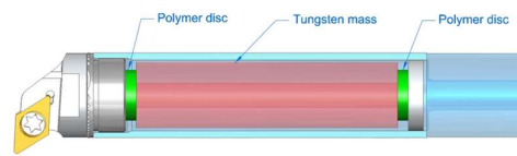
5 th Generation – from MAQ Polymers with frequency dependent stiffness
