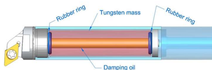
4 th Generation – Rubber rings with damping oil
