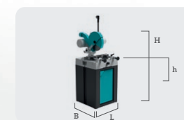
VELOX 350 B 610 mm L 880 mm H 990 mm h 895 mm Kg 163
