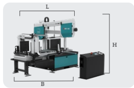
H 651 NC F 1000 B 2650 mm L 2900 mm H 2100 mm h 820 mm Kg 2300
