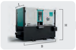
XSMART 4 B 3000 mm L 2600 mm H 2200 mm h 890 mm Kg 2800
