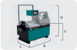
VELOX 350 AF-NC B 1800 mm L 1450 mm H 1950 mm h 930 mm Kg 607
