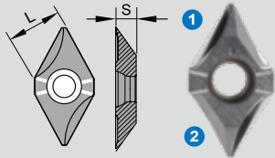
3 flutes, 2 cutting edges
